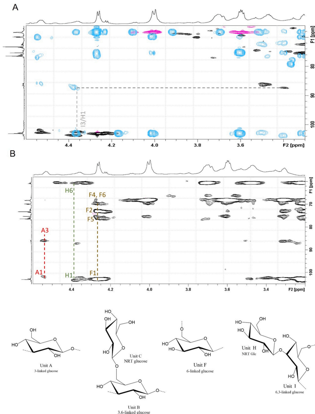
Fig. 4. NMR spectra of PEA2-SP. Superposition of HSQC (black) and HMBC (blue) spectra (A). Units identified in PEA2-SP (B). The pink correlations in panel A correspond to the HSQC correlations arising from position 6.
